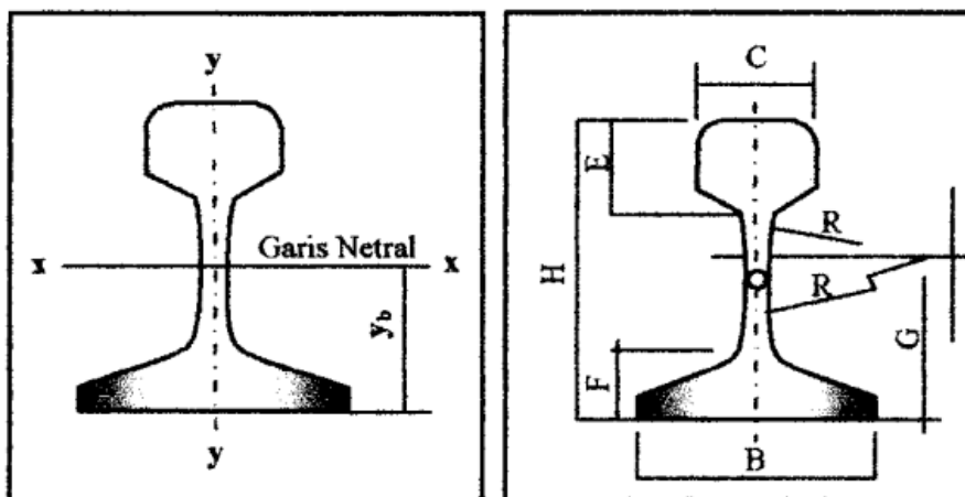
Gambar 1. Penampang Rel
