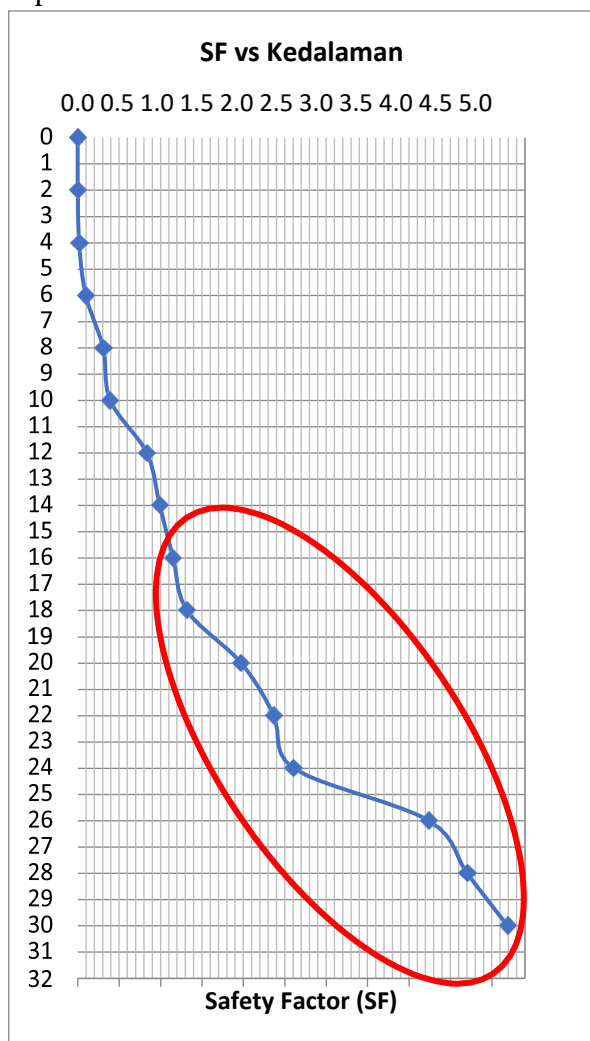
Gambar 6: Grafik SF vs Kedalaman BH 01
