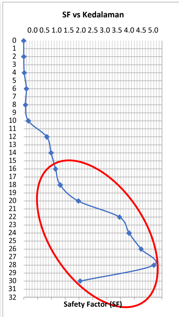
Gambar 7: Grafik SF vs Kedalaman BH 02
